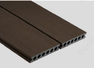
EPD06 Size: 145x21 mm Joist span: 350 mm Application: Residential use
