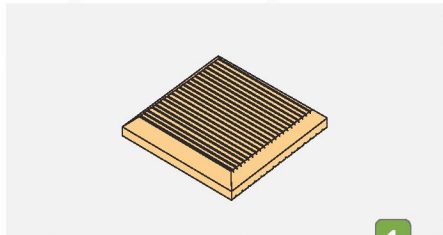
WPC Post Cap Code: IFS-CC Quantity: 2 pieces Size: 110*110*43mm
