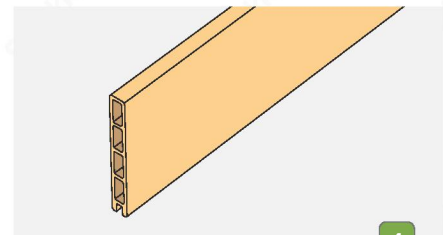
WPC Top Fencing Board Code: IFS-TB Quantity: 1 pieces Size: 1730*150*20mm
