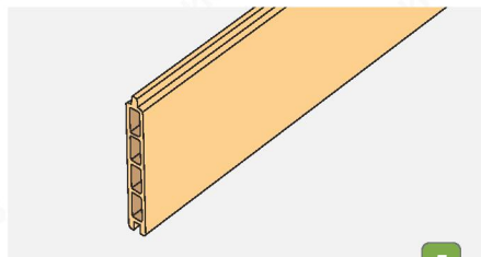
WPC Fencing Board Code: IFS-FB Quantity: 11 pieces Size: 1730*160*20mm
